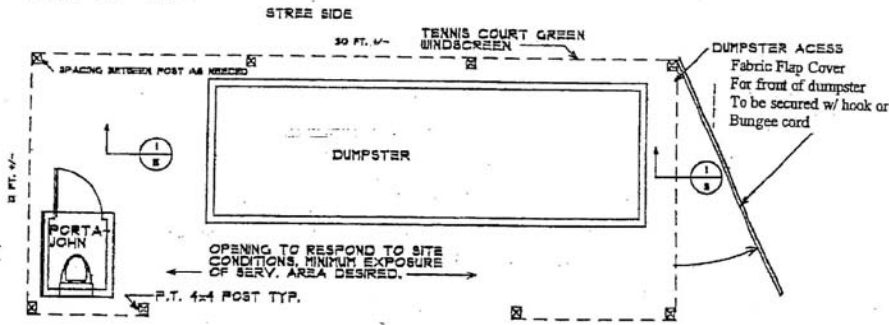
TYPICAL CONSTRUCTION SERVICE ENCLOSURE NOT TO SCALE
