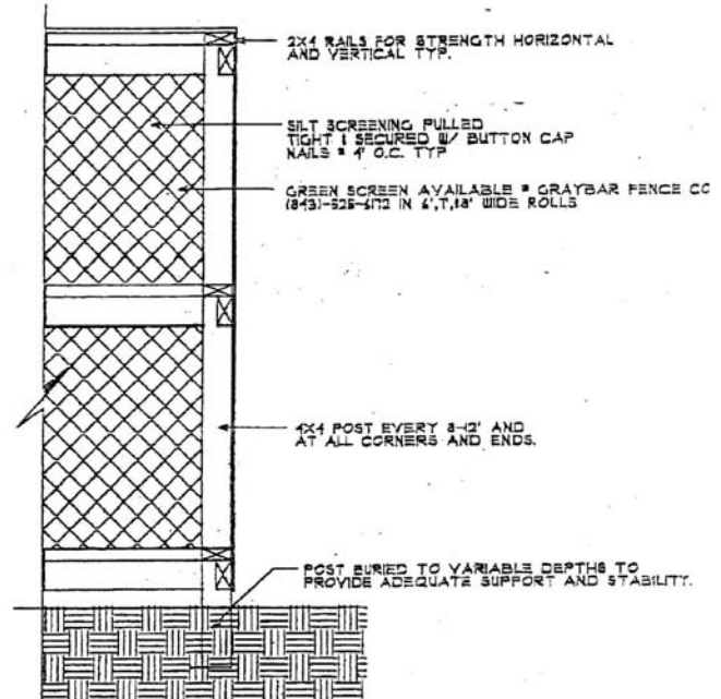
1 CROSS SECTION TYP. 2 NOT TO SCALE
